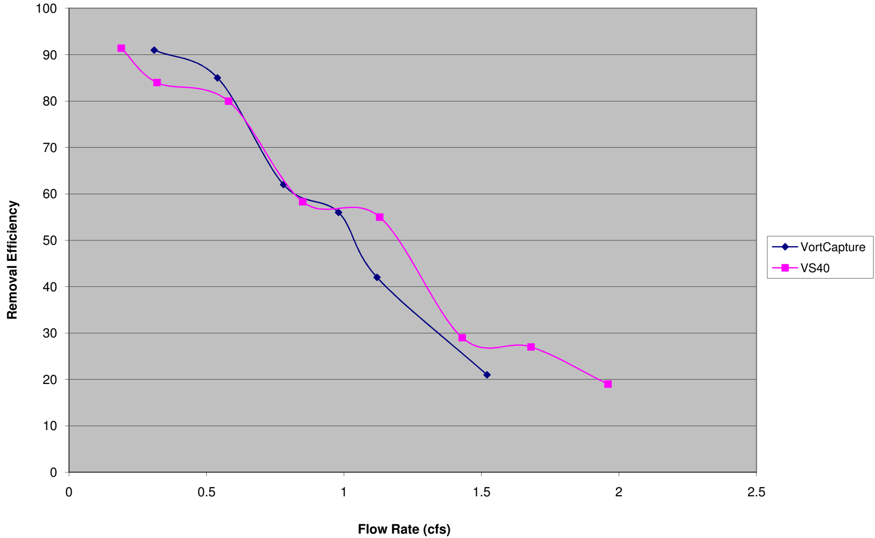
VS40 vs VortCapture Sediment Removal (OK-110)
