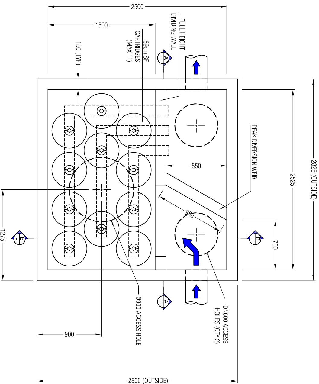
PLAN VIEW (LID OMITTED)
