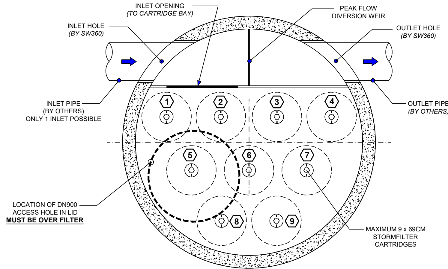
PLAN (ACCESS COVER AND LID REMOVED)
